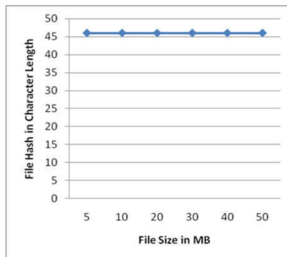
Figure 4.3. File Hash
