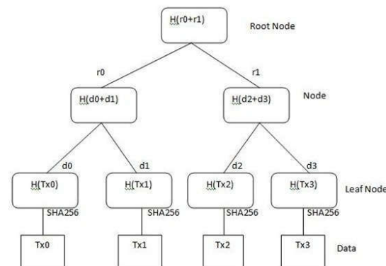
Figure 1.2: Merkle Tree
