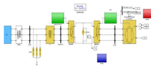
Fig.3. Simulation Circuit_WECS response at steady state for wind speed at 12 m/s
