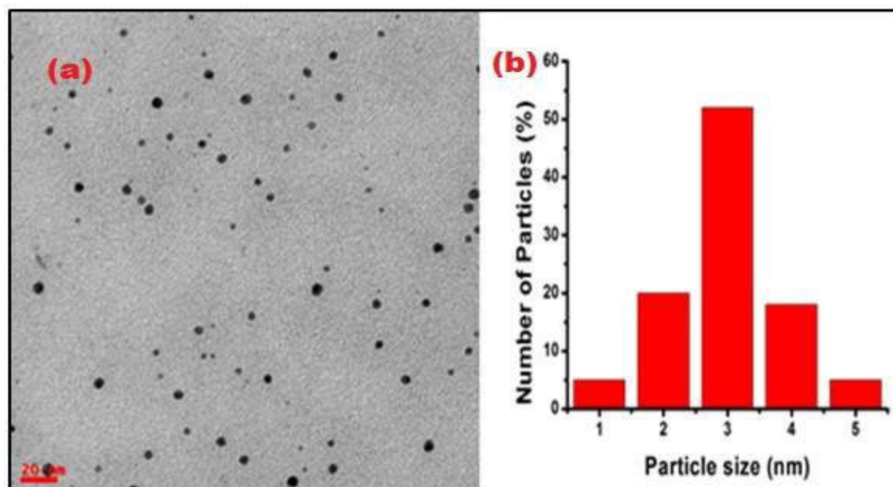
Figure: 4 (a)TEM analysis of GKPdNP (b) Histogram
